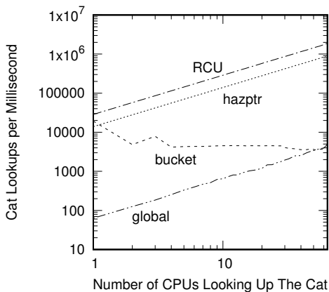
Figure 10.9: Read-Side Cat-Only RCU-Protected Hash-Table Performance For Schrödinger's Zoo at 64 CPUs
