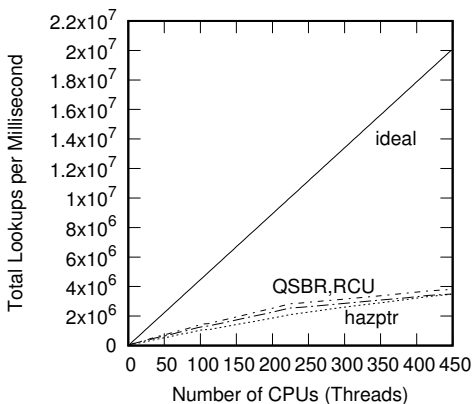
Figure 10.7: Read-Only RCU-Protected Hash-Table Performance For Schrödinger’s Zoo including QSB, Linear Scale
