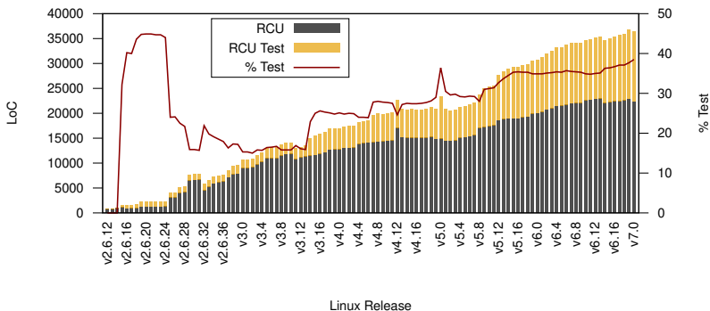
Figure 12.4: Linux-Kernel RCU Test Code
