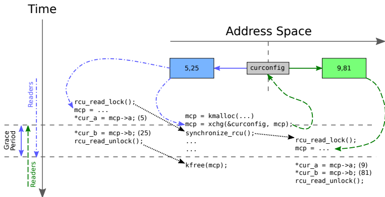
Figure 9.30: RCU Spatial/Temporal Synchronization
