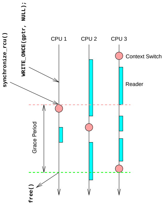
Figure 9.9: QSB: Waiting for Pre-Existing Readers
