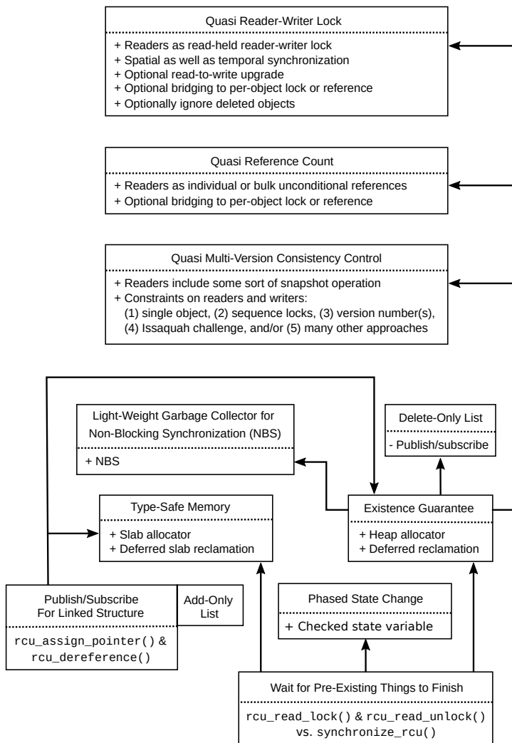
Figure 9.24: Relationships Between RCU Use Cases
