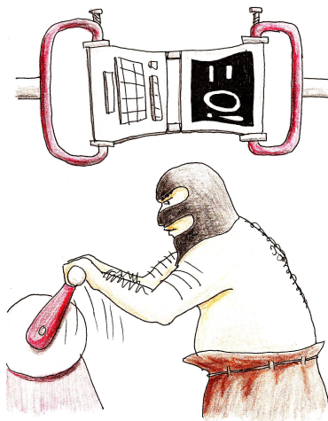
Figure 11.2: Rationalizing Validation
