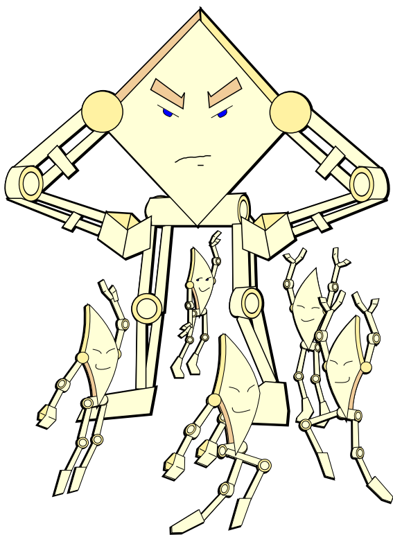
Figure 17.5: Astounding Accelerators
