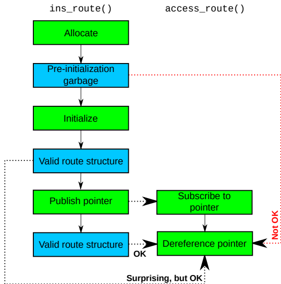
Figure 9.11: Publication/Subscription Constraints
