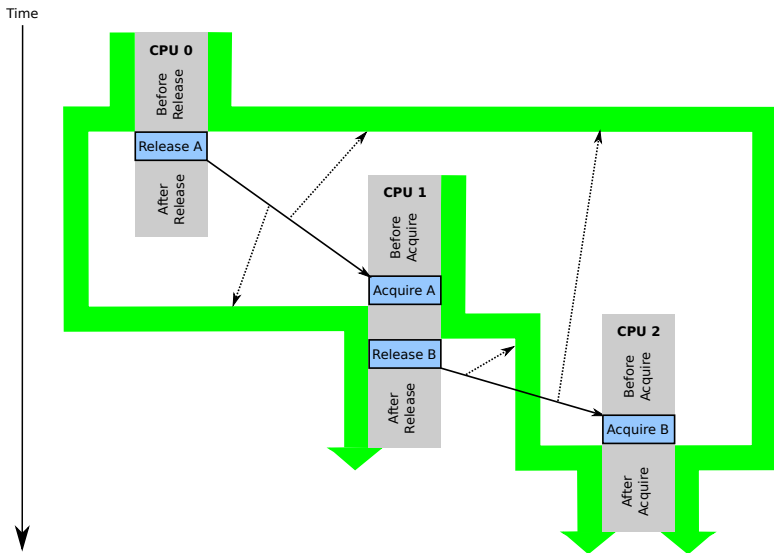
Figure 15.2: Release-Acquire Intuitions
