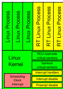
Figure 14.7: Linux-Kernel Real-Time Implementations
