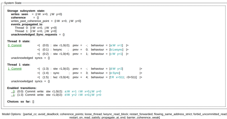
Figure 15.19: PPCMEM First R Step
