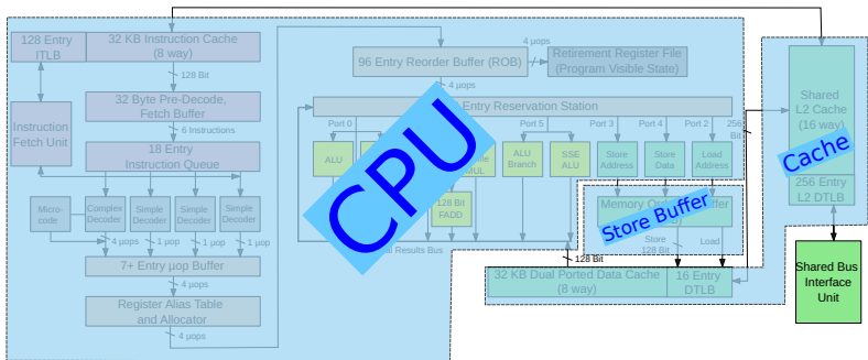
Figure 15.5: Intel Core 2 Architecture Simplified
