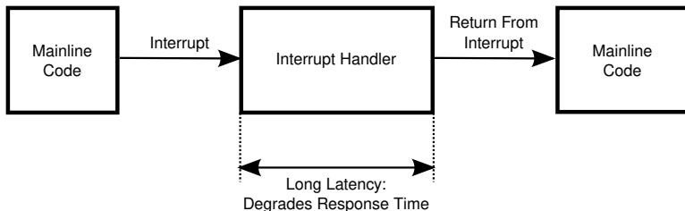
Figure 14.12: Non-Threaded Interrupt Handler
