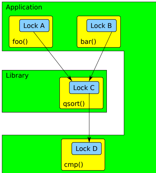
Figure 7.7: Layered Locking Hierarchy for qsort()
