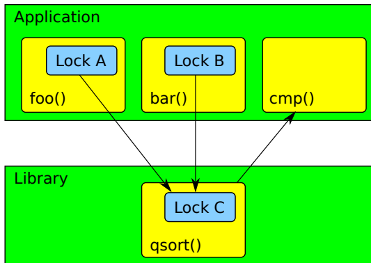
Figure 7.4: No qsort() Compare-Function Locking
