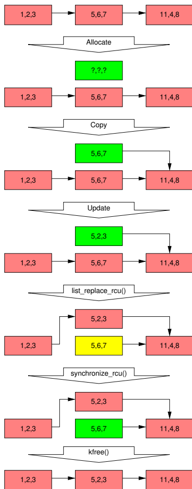
Figure 9.20: RCU Replacement in Linked List
