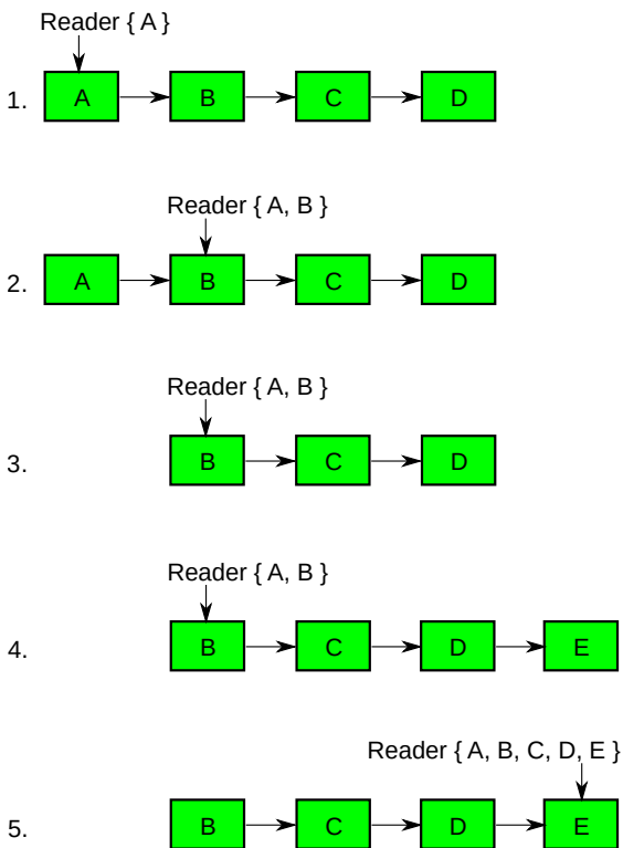
Figure 9.16: Multiple RCU Data-Structure Versions
