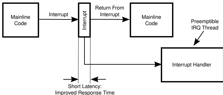
Figure 14.13: Threaded Interrupt Handler
