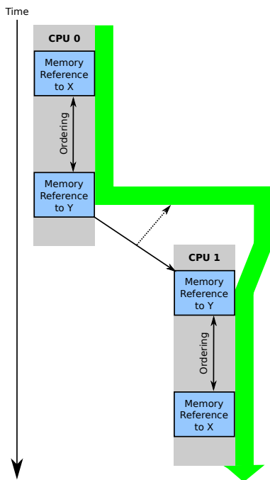
Figure 15.3: If-Then Nature of Memory Ordering
