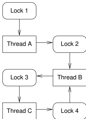
Figure 7.3: Deadlock Cycle
