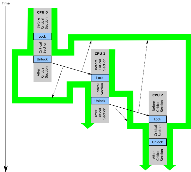
Figure 15.1: Locking Intuitions
