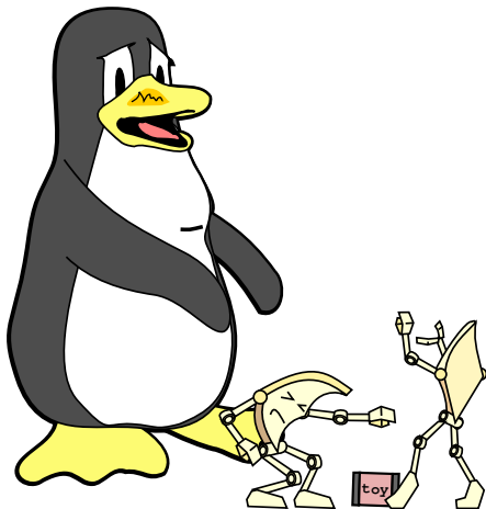
Figure 6.13: Lock Contention
