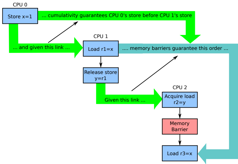
Figure 15.14: Cumulativity
