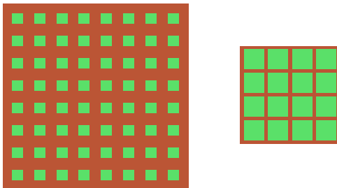
Figure 2.6: Coarse Partitioning Reduces Synchronization Overhead
