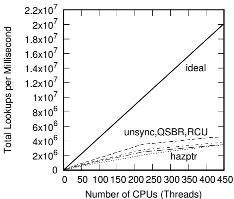
Figure 10.8: Read-Only RCU-Protected Hash-Table Performance For Schrödinger’s Zoo including QSB and Unsynchronized, Linear Scale
