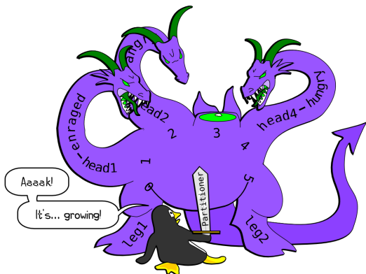
Figure 10.13: Partitioning Problems
