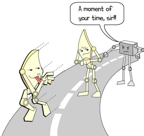
Figure 3.11: CPU, Interrupted
