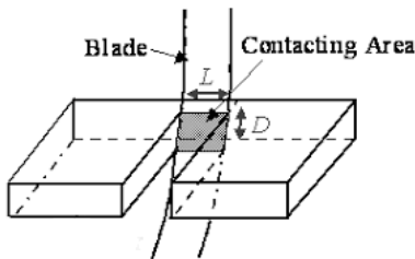
Figure 7.9: Saw Kerf
