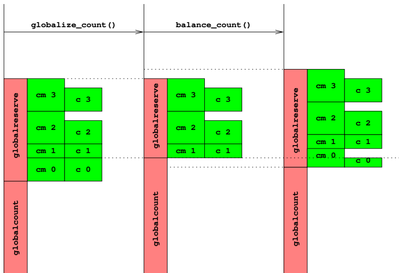
Figure 5.6: Schematic of Globalization and Balancing
