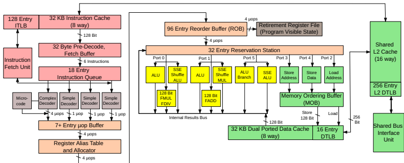
Figure 15.4: Intel Core 2 Architecture
